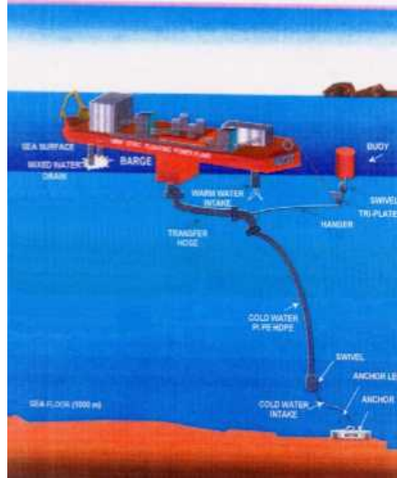
OCEAN. THERMAL. ENERGY. CONVERSION. CONCEPTUAL. DIAGRAM
